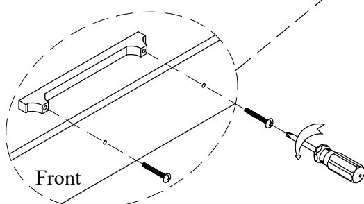
Remove Handle from inside drawer
